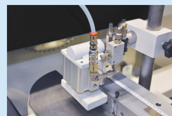
Vertical pneumatic clamp
