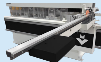
Automatic length-fence
